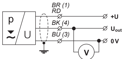
(X) – Connector terminal numbers
