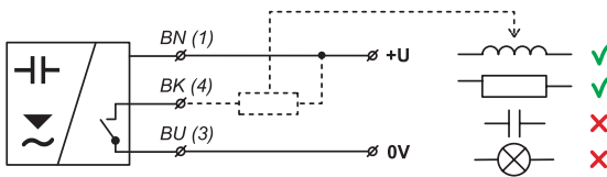
Fig. 11: NPN output type sensor connection (configuration N, NT)
